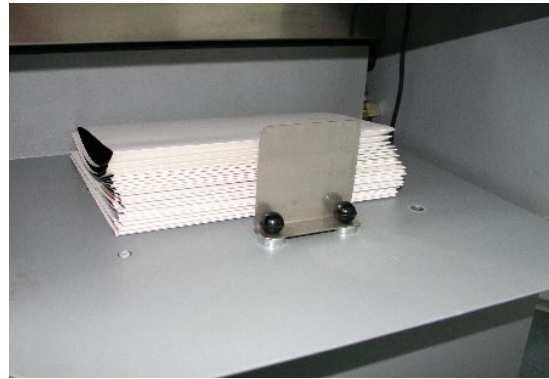
In an automatic working cycle all pages will be automatically creased and folded, and after this transported and stapled into a collection area.
